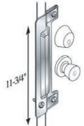
11-3/4" LATCH GUARD Fits single & double locks up to 6" on center. MG-8850C MG-8850DU
