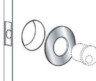
ADAPTER PLATE 2 5/8" DIA FOR RIM OR MORTISE CYLINDERS COVERS UP TO 2 1/8" DIA. HOLE
