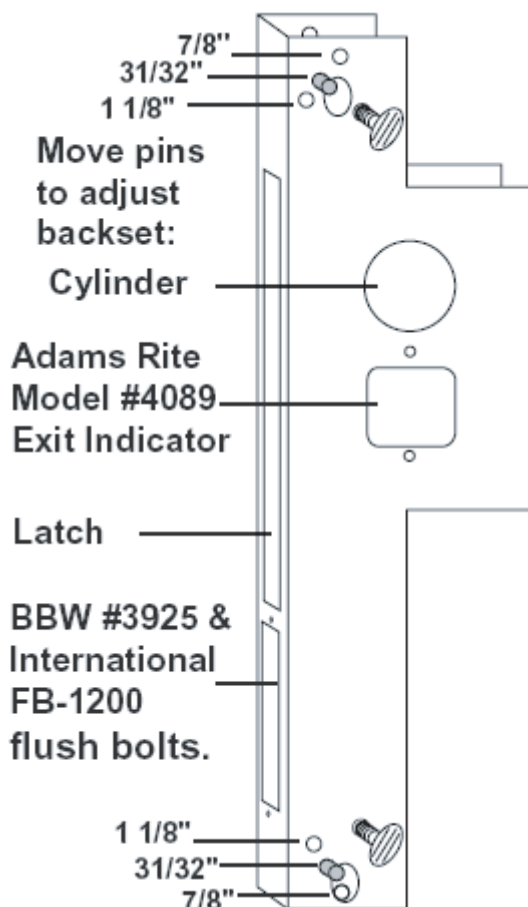
KX-TMPA/R ADAMS RITE INSTALLATION TEMPLATE
