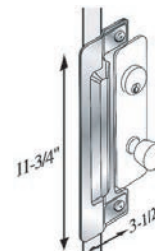
11-3/4" UNIVERSAL LATCH GUARD Out-Opening Doors, with 1" x 8-3/4" Cutout MG-8849DU
