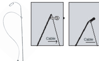
KX-K-22 LEVER OPENING TOOL
