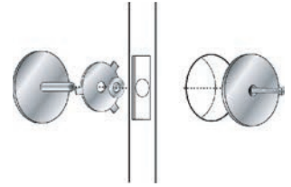
HOLE COVER 2 5/8" DIA. COVERS 1/2" TO 2 1/8" HOLES
